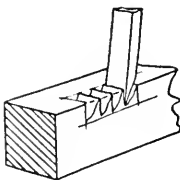
FIG. 443. RABBETING WITH CHISEL.
